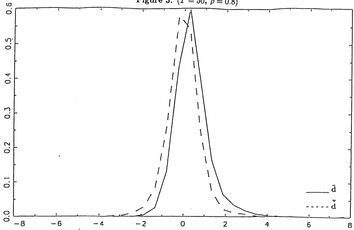
Figure 3. ( T = 50, \rho = 0.8 )
