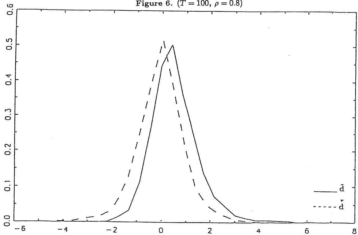
Figure 6. ( T = 100, \rho = 0.8 )
