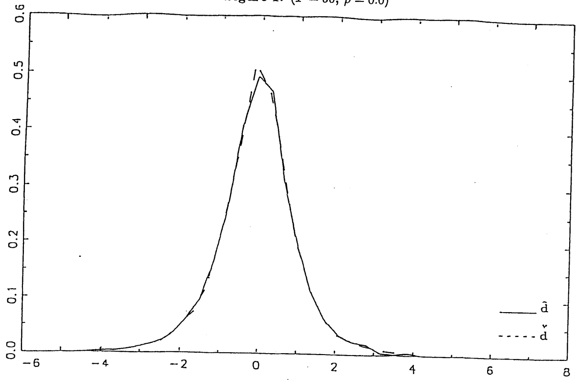
Figure 1. ( T = 50, \rho = 0.0 )
