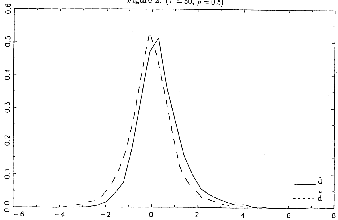
Figure 2. ( T = 50, \rho = 0.5 )
