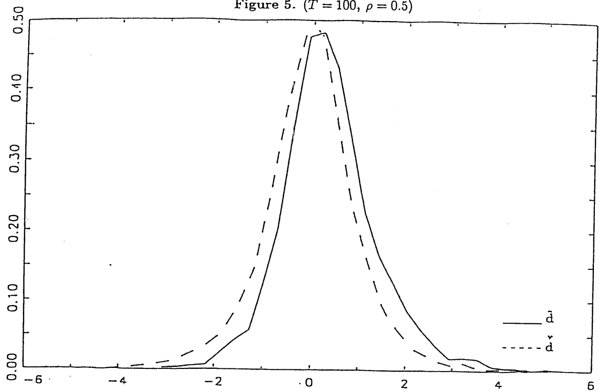
Figure 5. ( T = 100, \rho = 0.5 )
