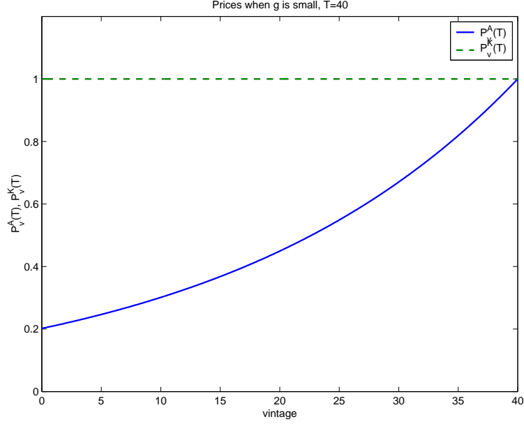
Figure 4: Prices of capital in the case \hat{q} < \alpha(\delta^B - \delta^A) , where the investment scheme is (c) \forall v .
