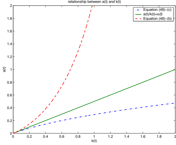
Figure 1: Possible per effective long-lived capital, a(t) , and short-lived capital, b(t) implied by (8) when \hat{q} > \alpha(\delta^B - \delta^A) .
