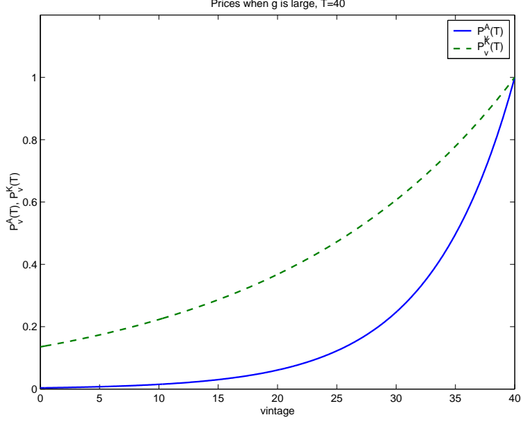
Figure 3: Prices of capital in the case \alpha(\delta^B - \delta^A) < \hat{q} , where the investment scheme is (a) \forall v .
