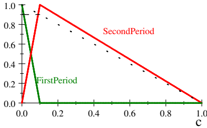
Figure 1: Two period trade for e^{-r\Delta} = 0.9 .
