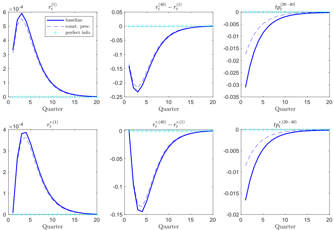
Figure 11: Impulse Responses to \varepsilon_{s,t} — term structure
