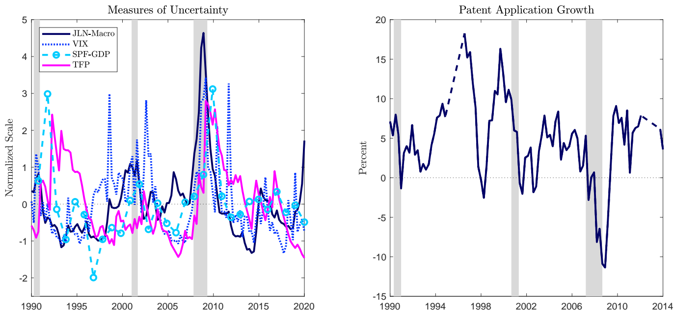
Figure 2: Measures of Uncertainty and Information
