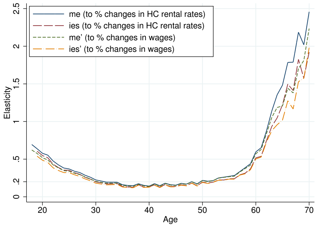
Figure 5a: Calculated elasticities
